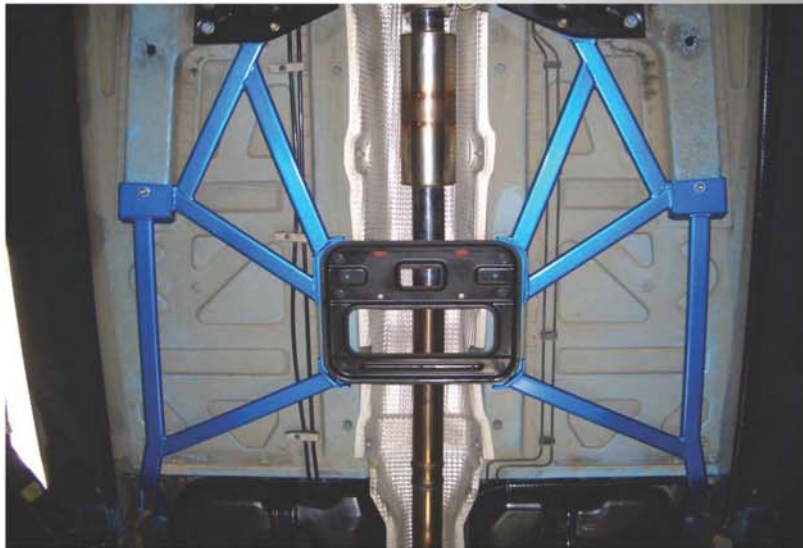
Undershot of mounting points front & rear power brace
