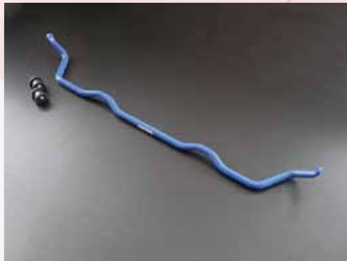
Front Sway Bar (692 311 A24) MSRP $334 (25,000 JPY)
